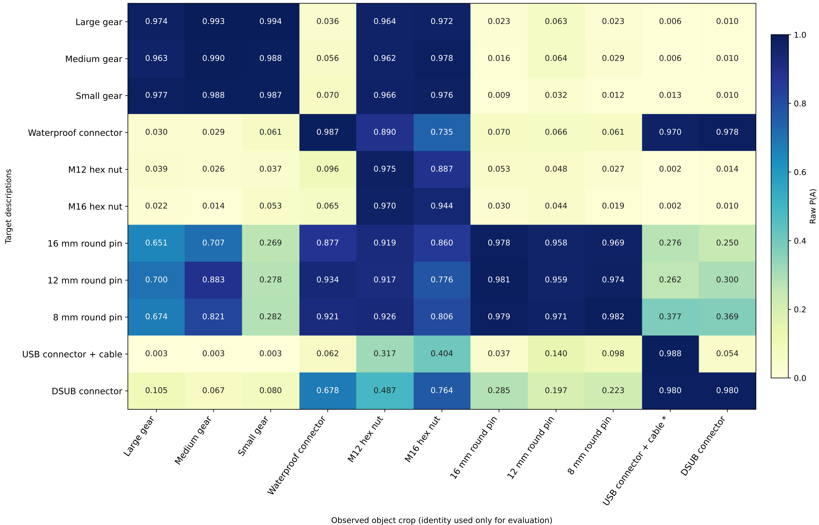
Scene 101: qwen3.5:9b raw P(A)
