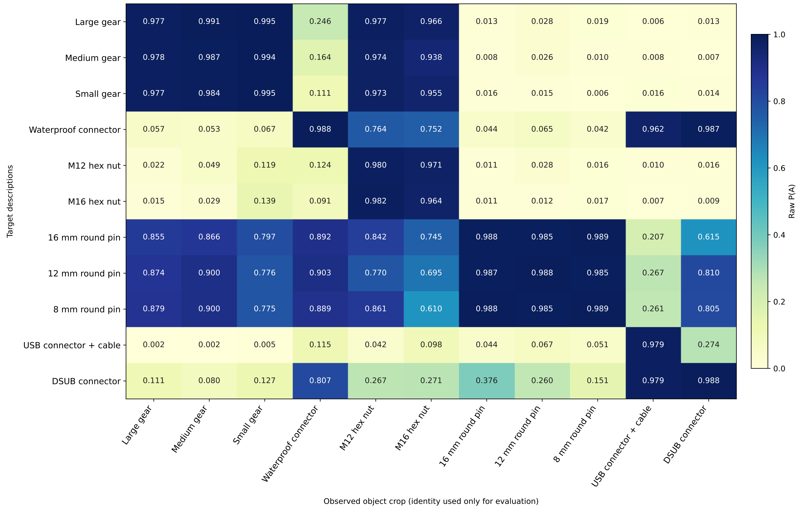
Baseline: qwen3.5:9b raw P(A)
