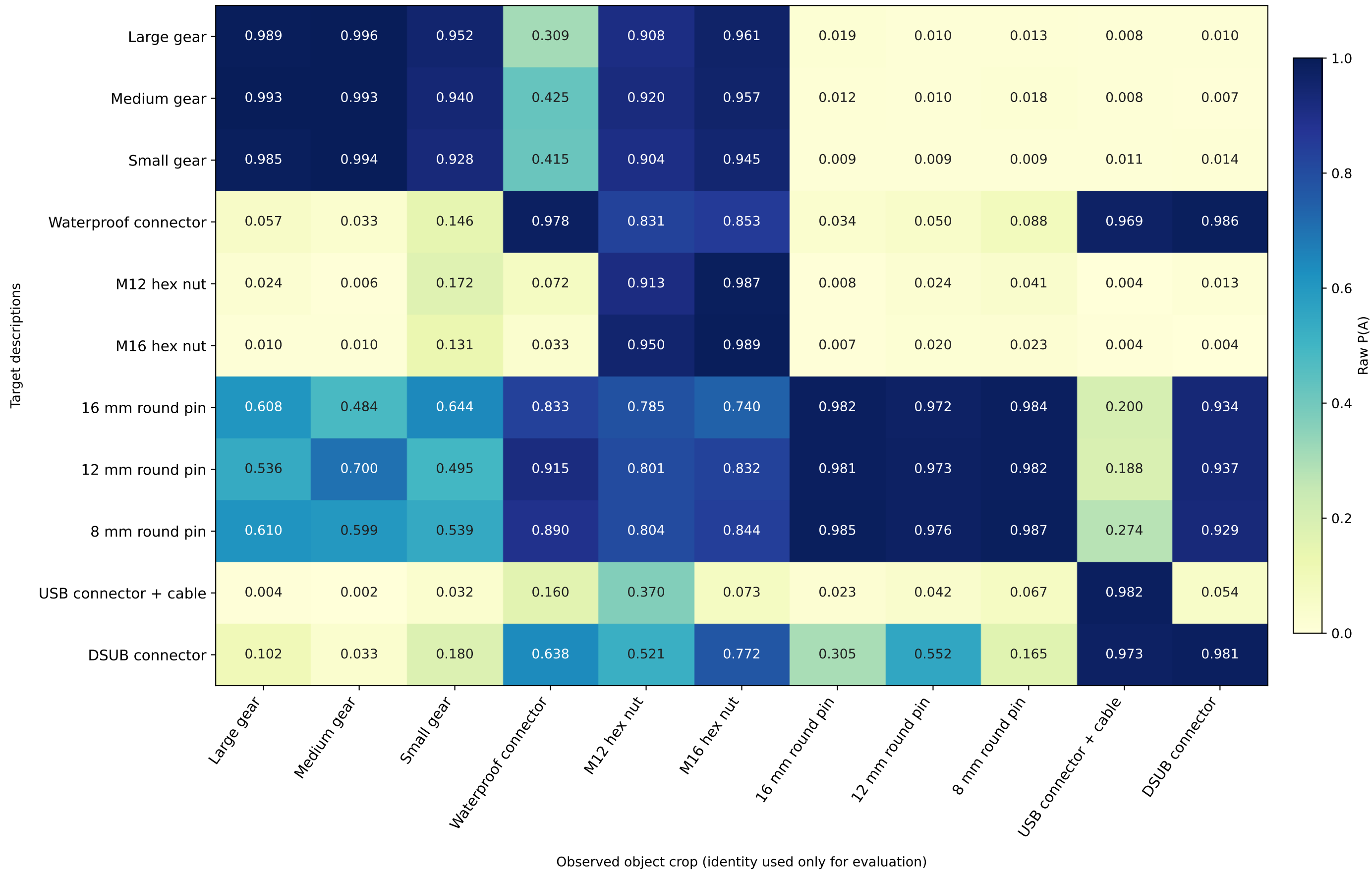
Scene 202: qwen3.5:9b raw P(A)
