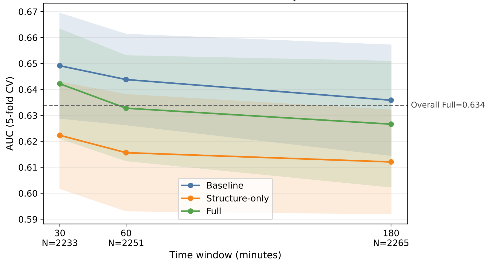
F1: Time-window Timeliness vs Veracity Performance
