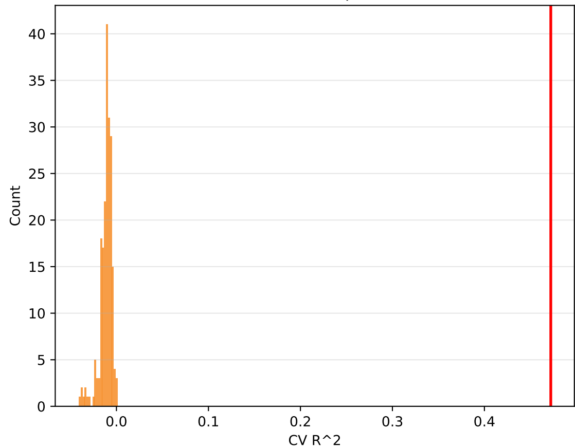
Reach R^2 null ( p=0.000 )
