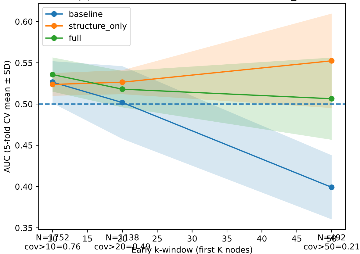
Veracity prediction (k-window, fixed valid set: final_size > K)
