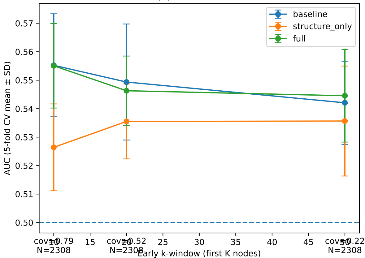
Veracity prediction (k-window)
