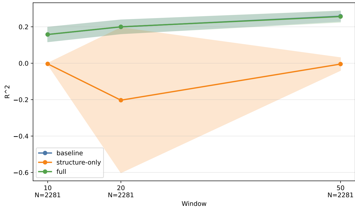
Reach ( R^2 ) vs K-window
