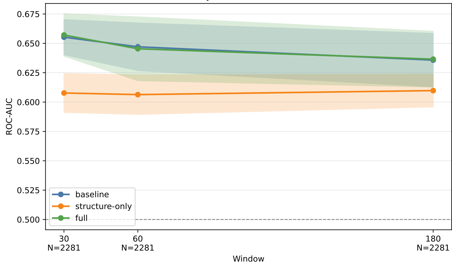
Veracity (AUC) vs Time Window
