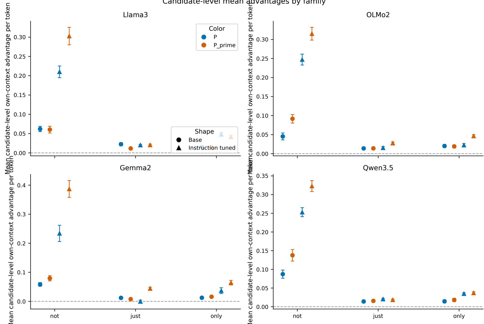
Candidate-level mean advantages by family
