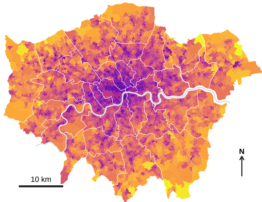
Grid-informed
