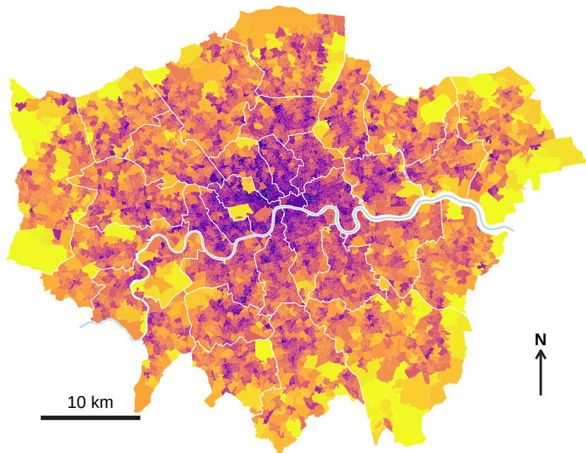
Centroid-based
