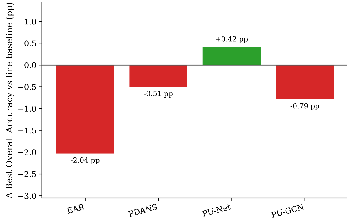
Line B: \Delta Best Overall Accuracy vs Downsampled x4 Baseline
