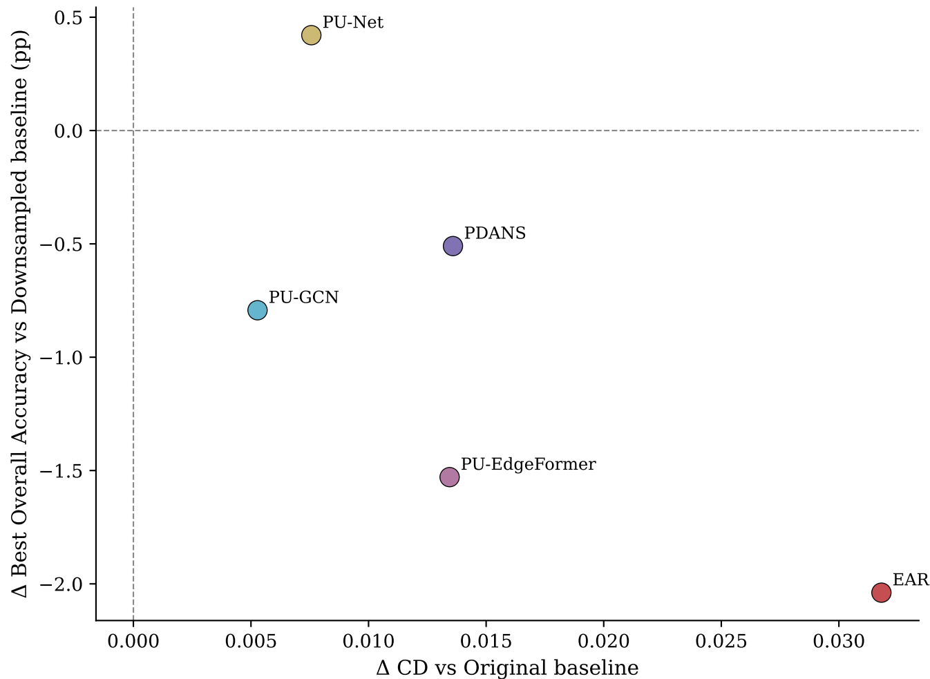
Line B: \Delta CD vs \Delta Classification (final)
