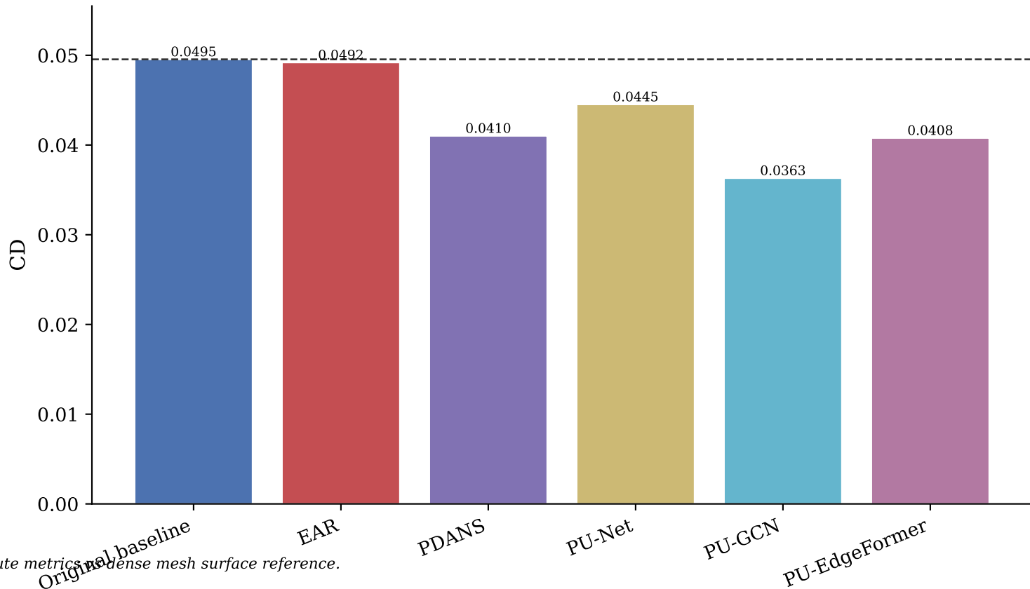
Line A absolute CD (supplementary)
