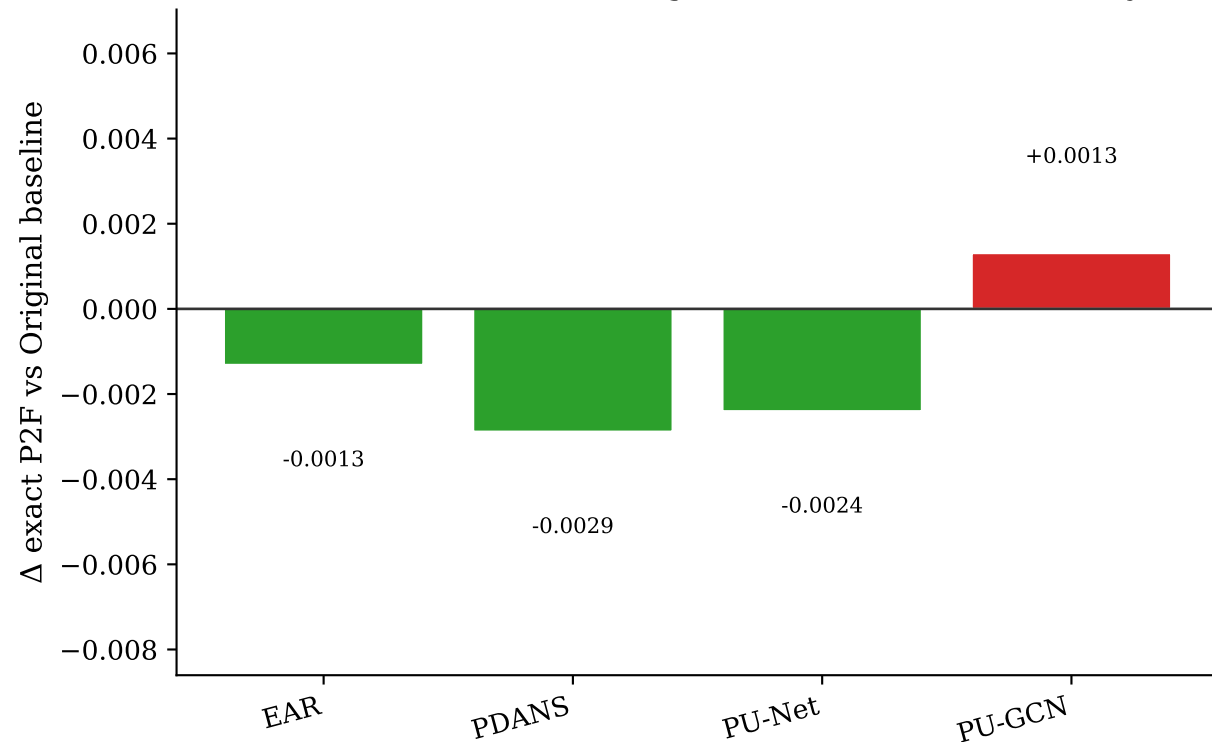
Line B: \Delta exact P2F vs Original Baseline (Methods Only)
