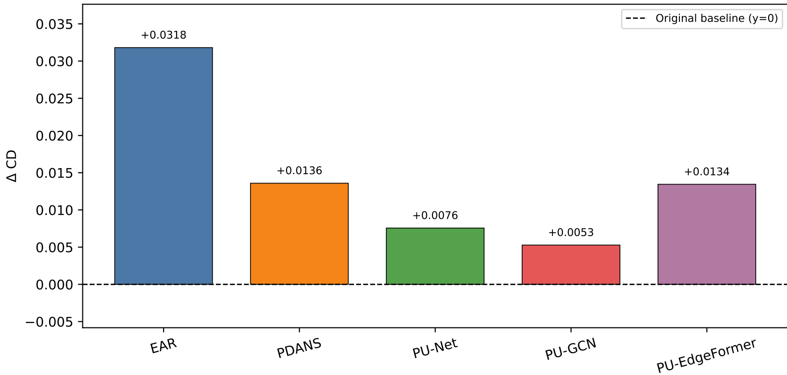
Line B \Delta CD vs Original baseline (methods only)
