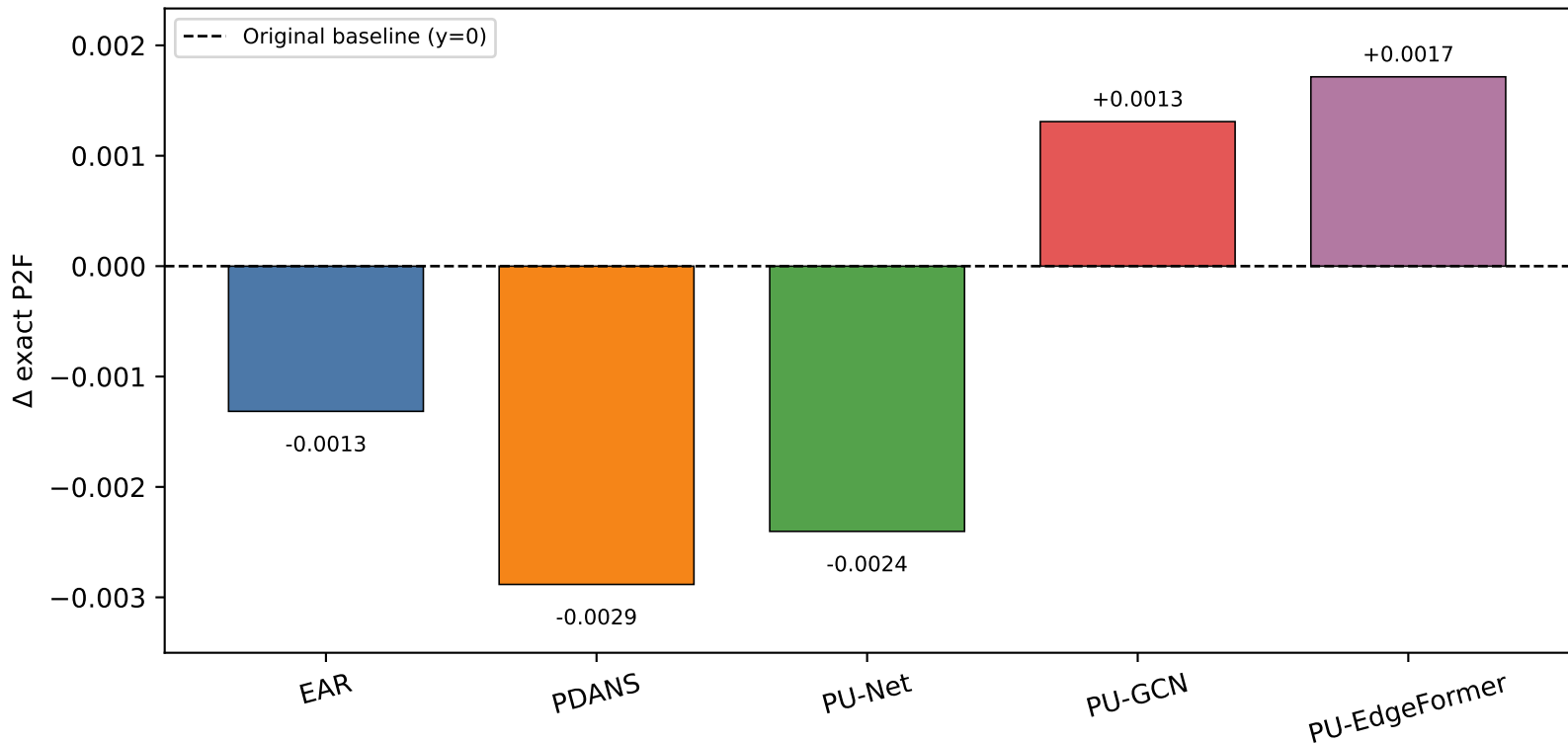
Line B \Delta exact P2F vs Original baseline (methods only)
