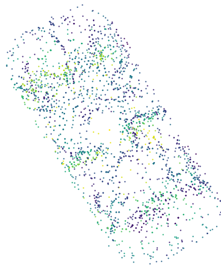
EAR 4096
