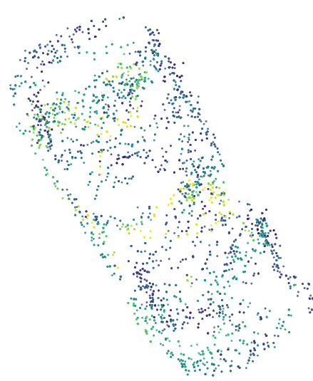
PU-Net 4096
