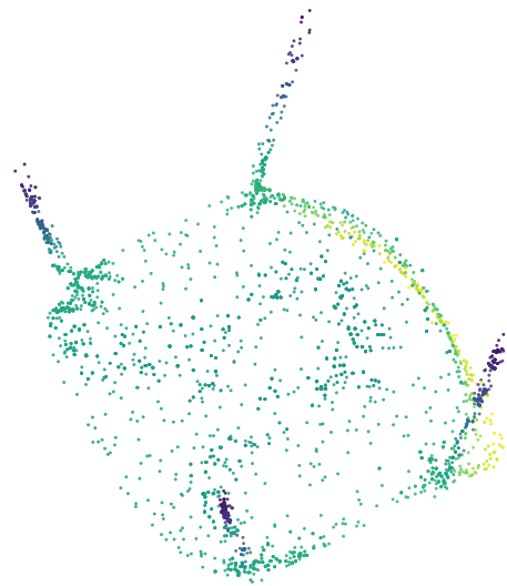
EAR 4096
