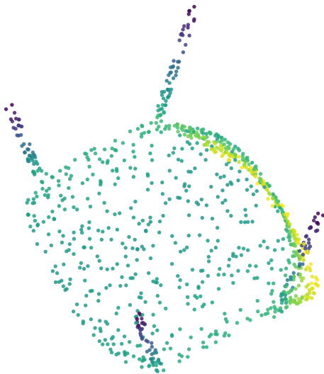
Original 1024
