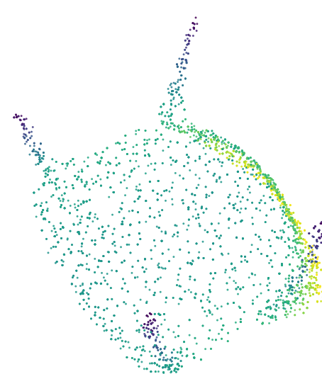
PU-Net 4096
