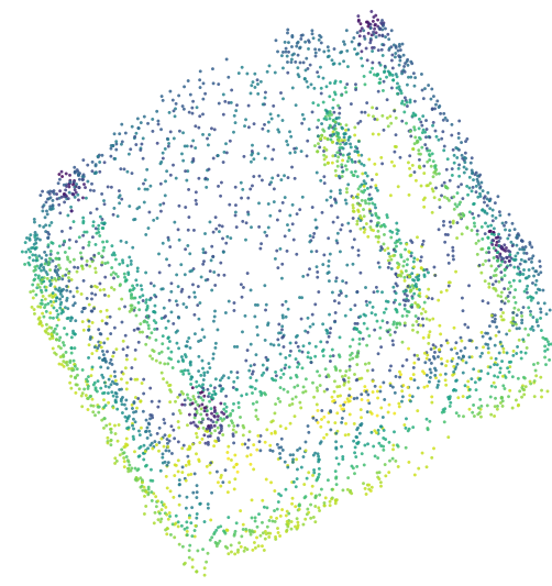
PU-Net 4096
