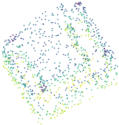
Original 1024
