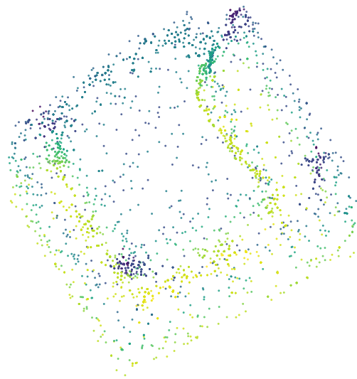
EAR 4096
