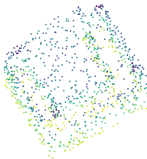
Original 1024
