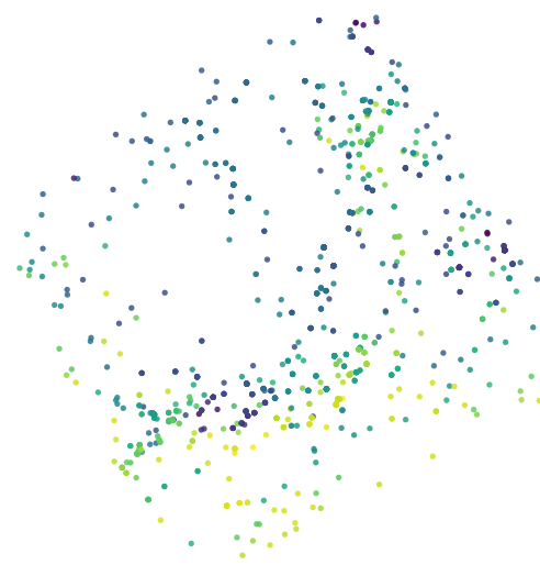
EAR 1024
