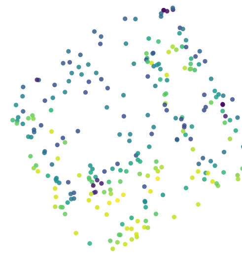
Downsampled x4 256
