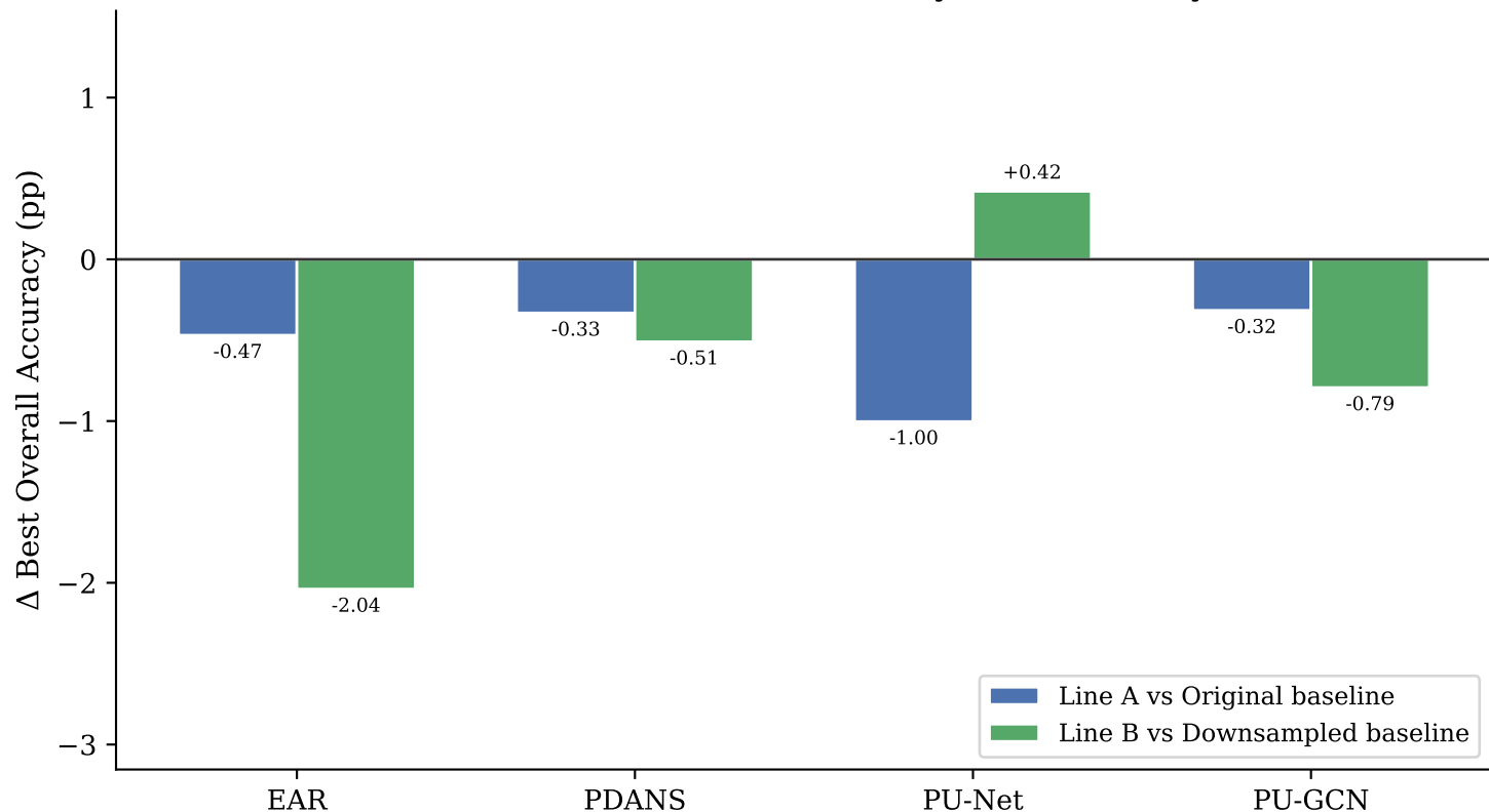
Two-Line \Delta Best Overall Accuracy (Methods Only)
