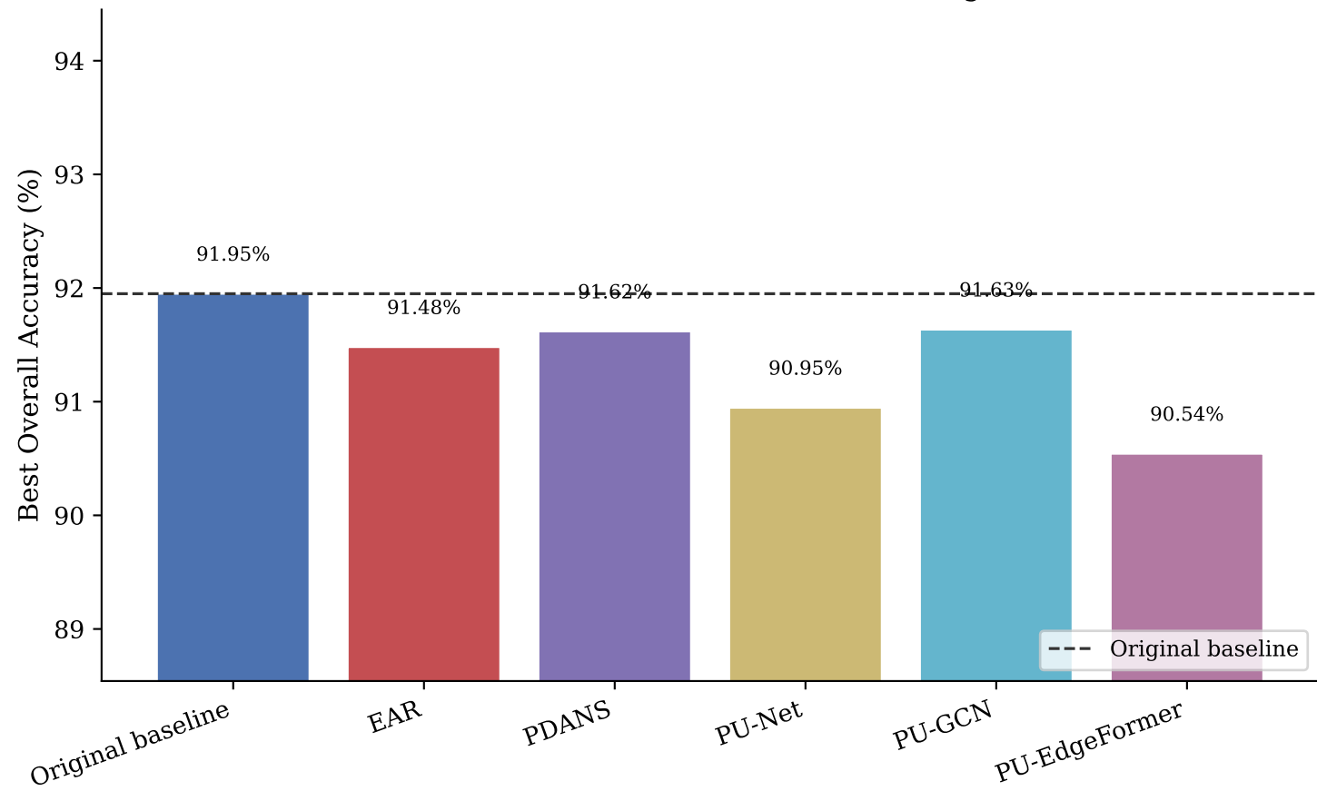
PointNet++ Line A Best Overall (with PU-EdgeFormer)
