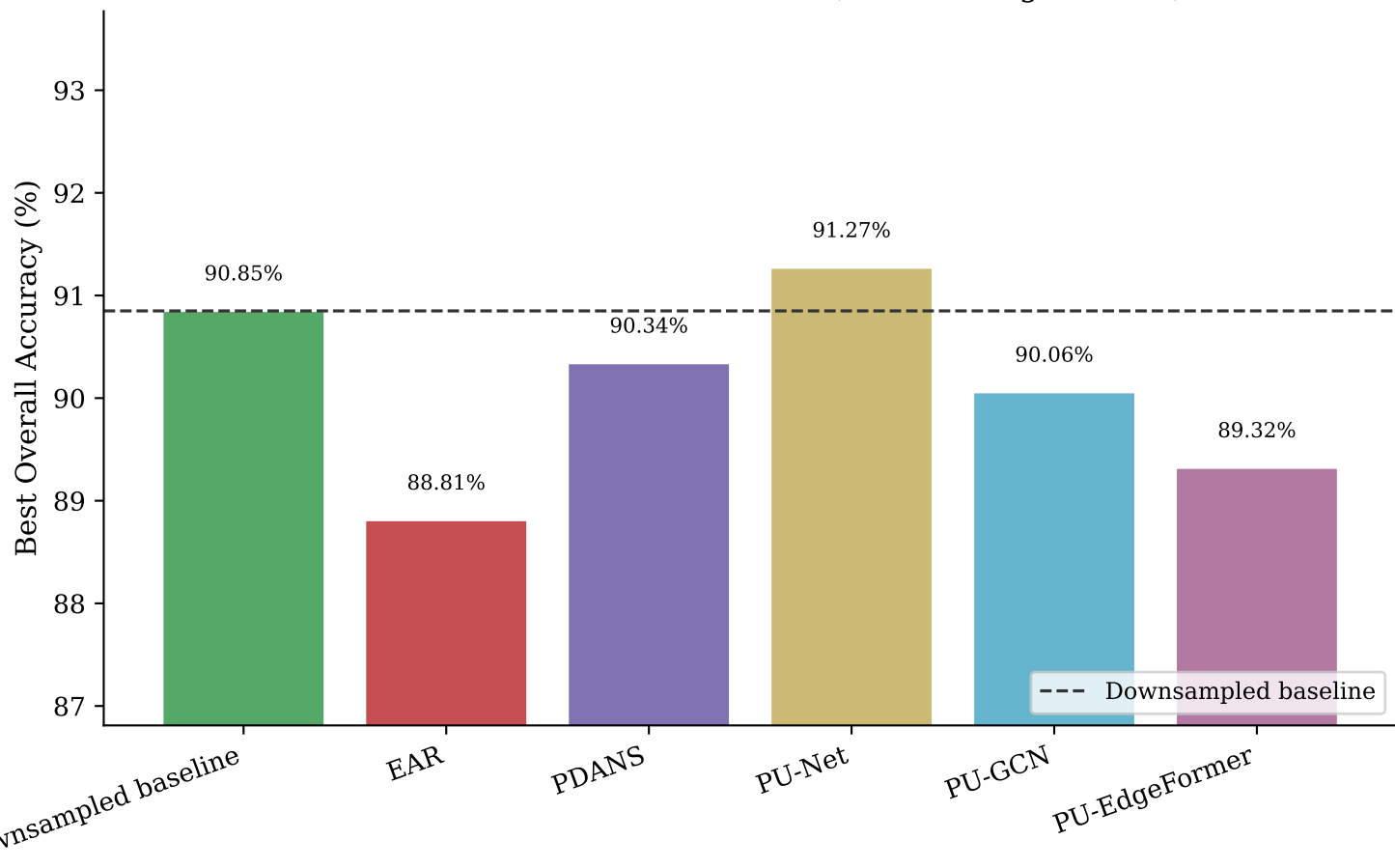
PointNet++ Line B Best Overall (with PU-EdgeFormer)
