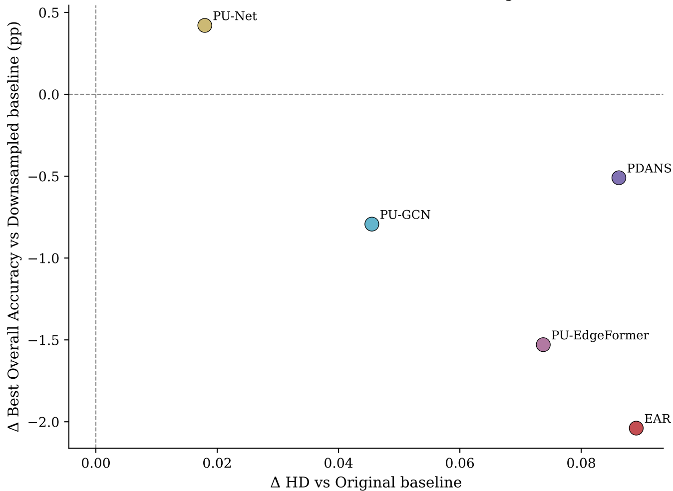
Line B: \Delta HD vs \Delta Classification (with PU-EdgeFormer)
