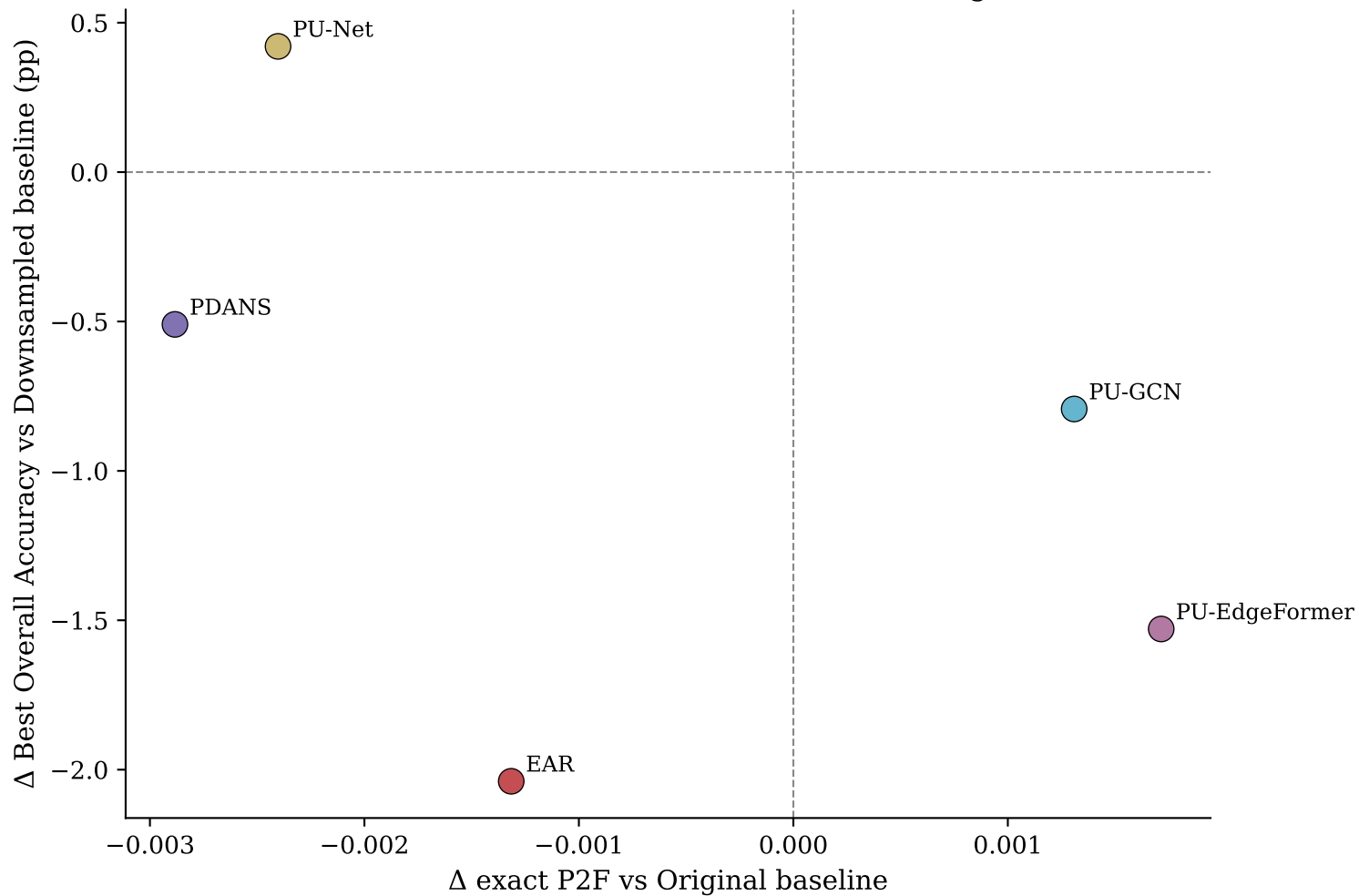
Line B: \Delta exact P2F vs \Delta Classification (with PU-EdgeFormer)
