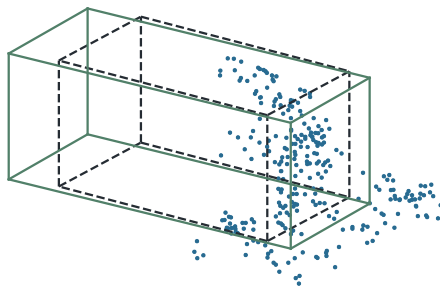
Upsampled TP: 3D IoU 0.705
