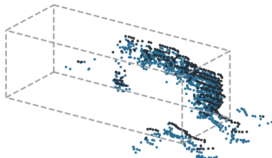
(e) PU-Net*
