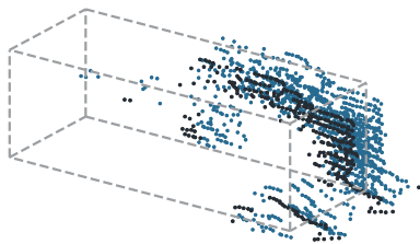
(e) PU-Net*
