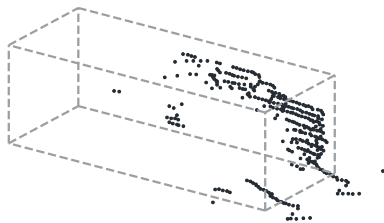
(c) PU-GCN
