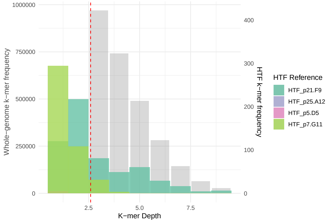
HTF & WG k-mer depth for 64.GBR_1933b_S36
