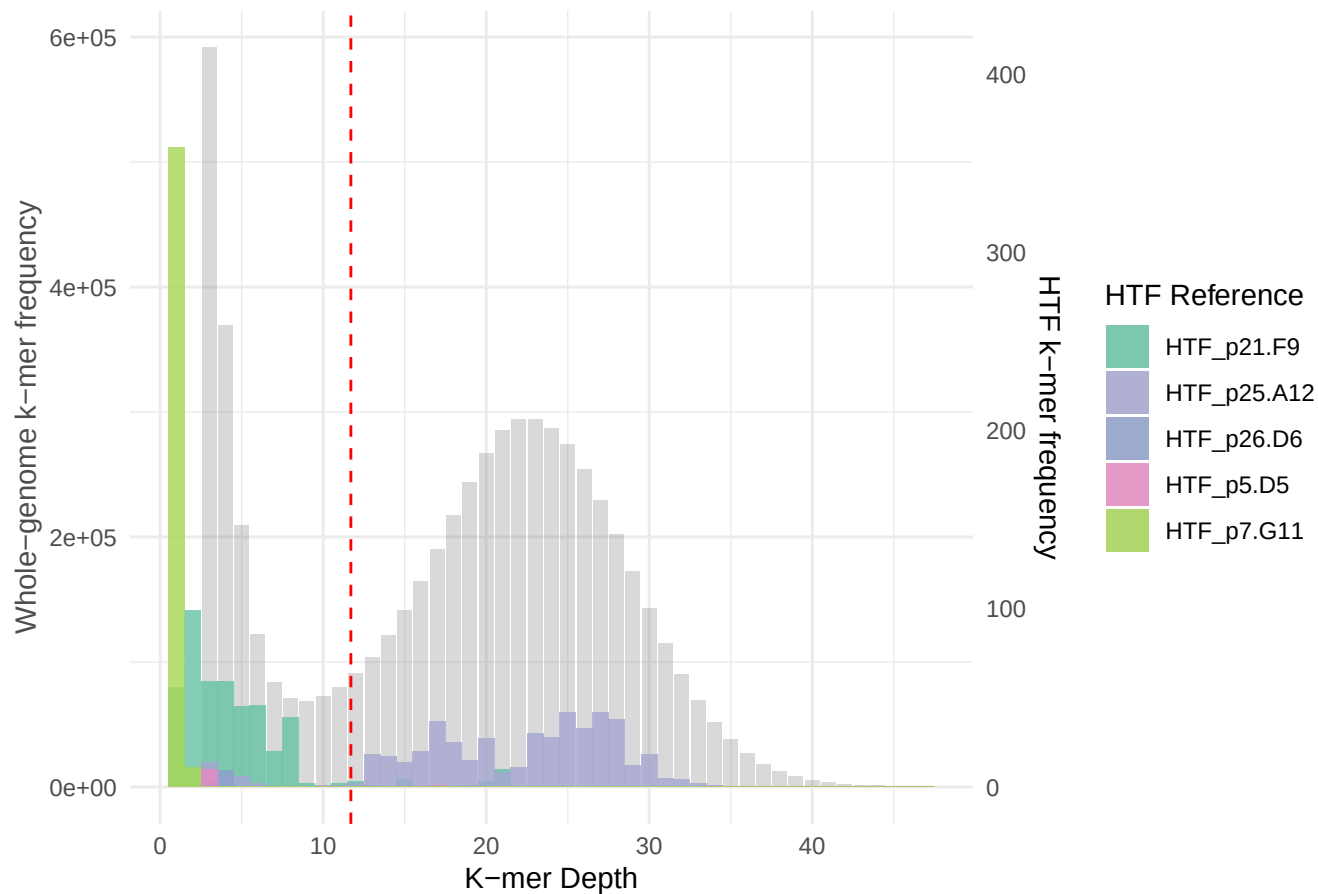
HTF & WG k-mer depth for PL0080
