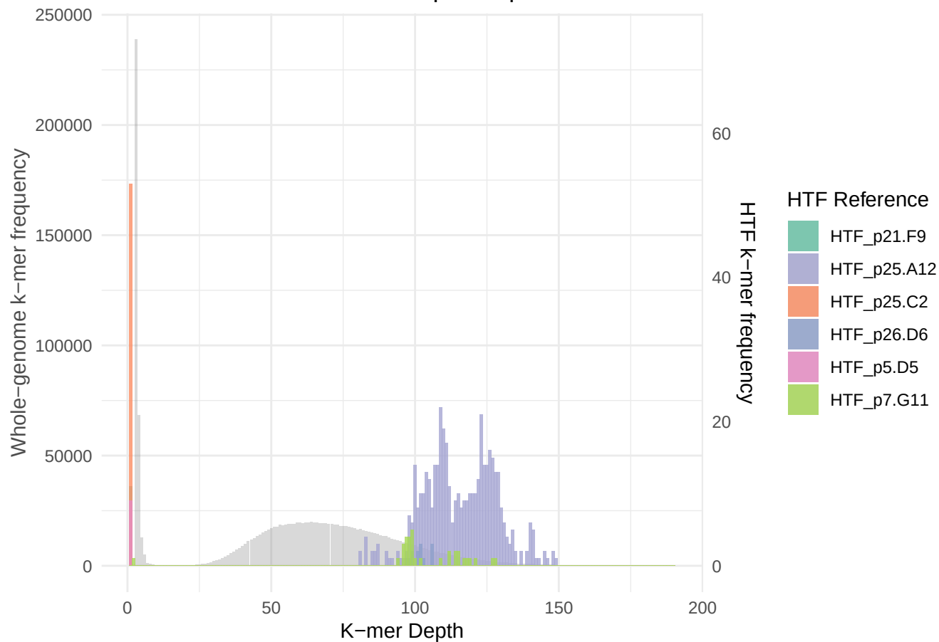
HTF & WG k-mer depth for p13.D10
