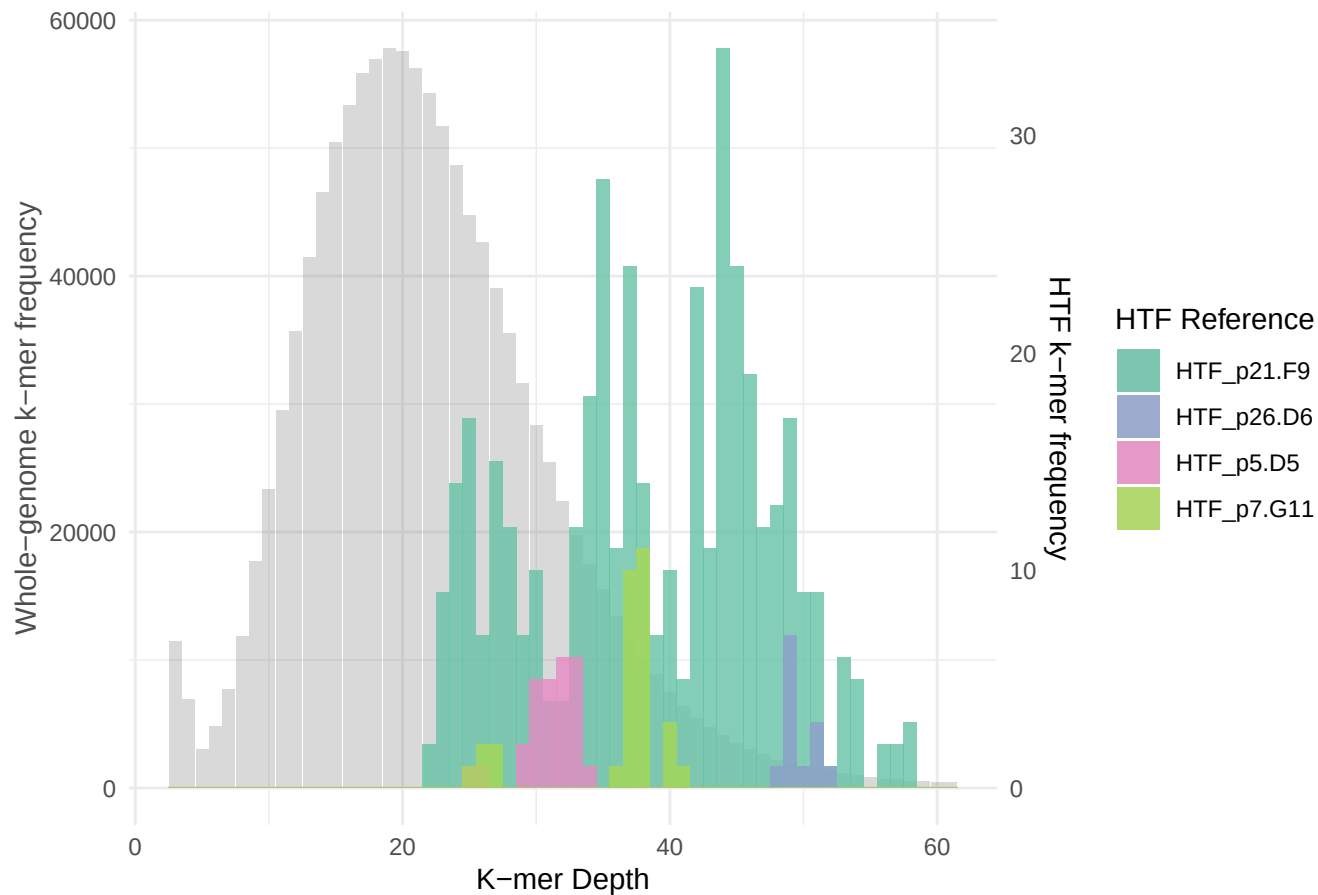
HTF & WG k-mer depth for p4.E6
