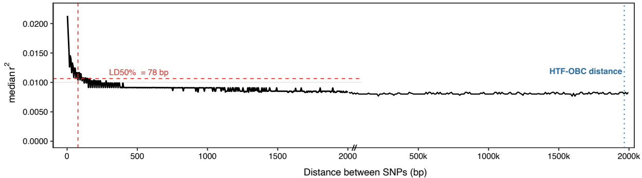
Genome-wide LD decay
