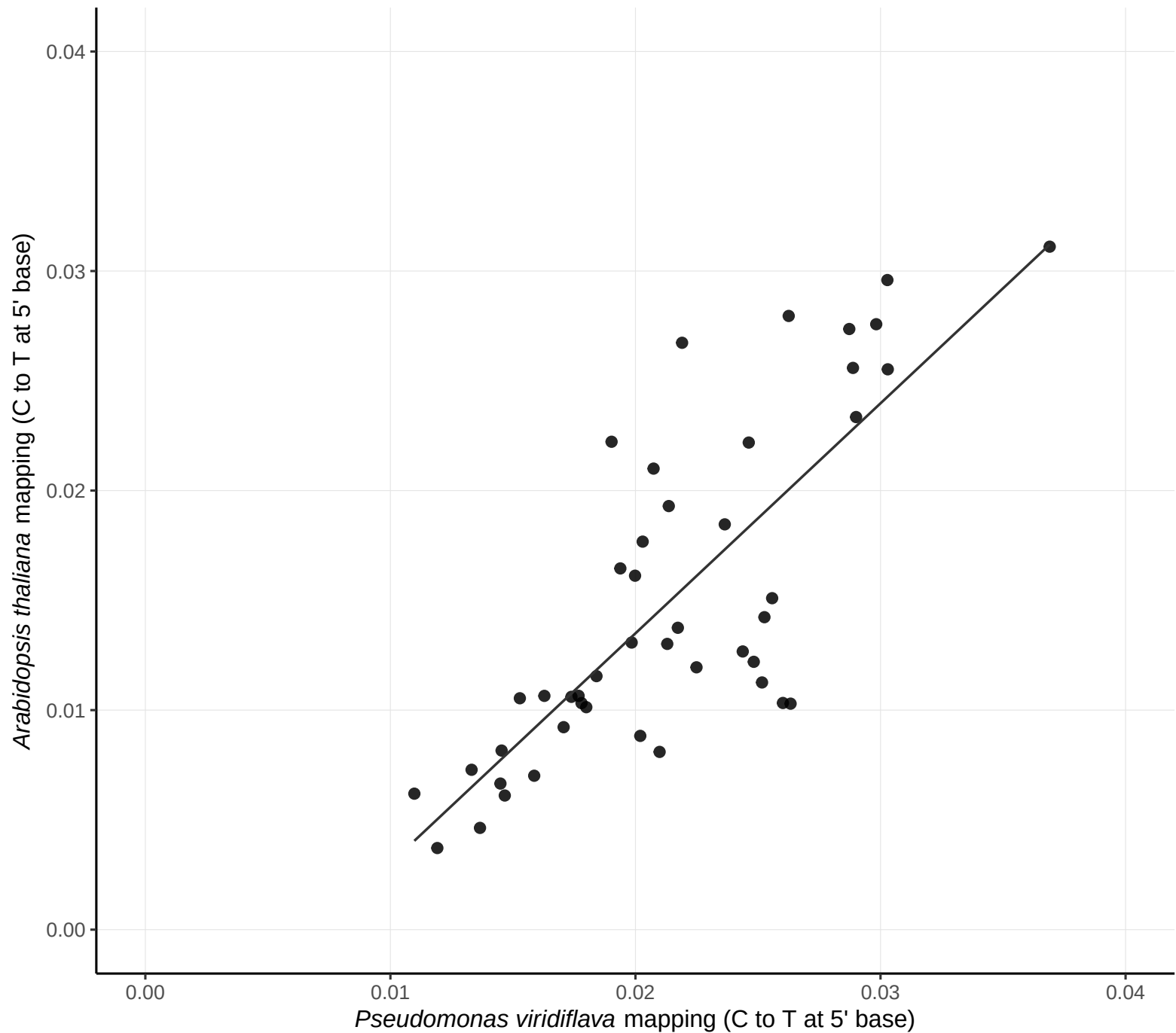
First-base C to T frequency: Pseudomonas viridiflava vs Arabidopsis thaliana
