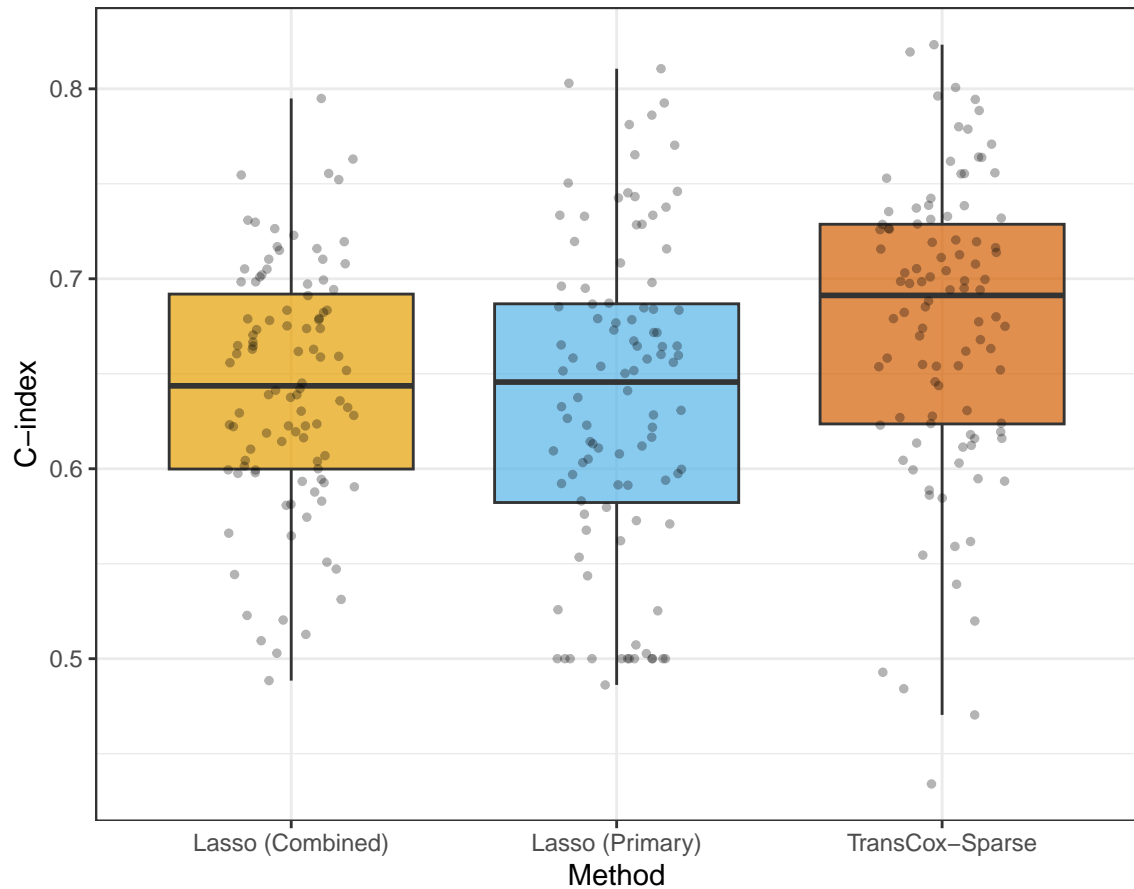
C-index Distribution (100 Runs)
