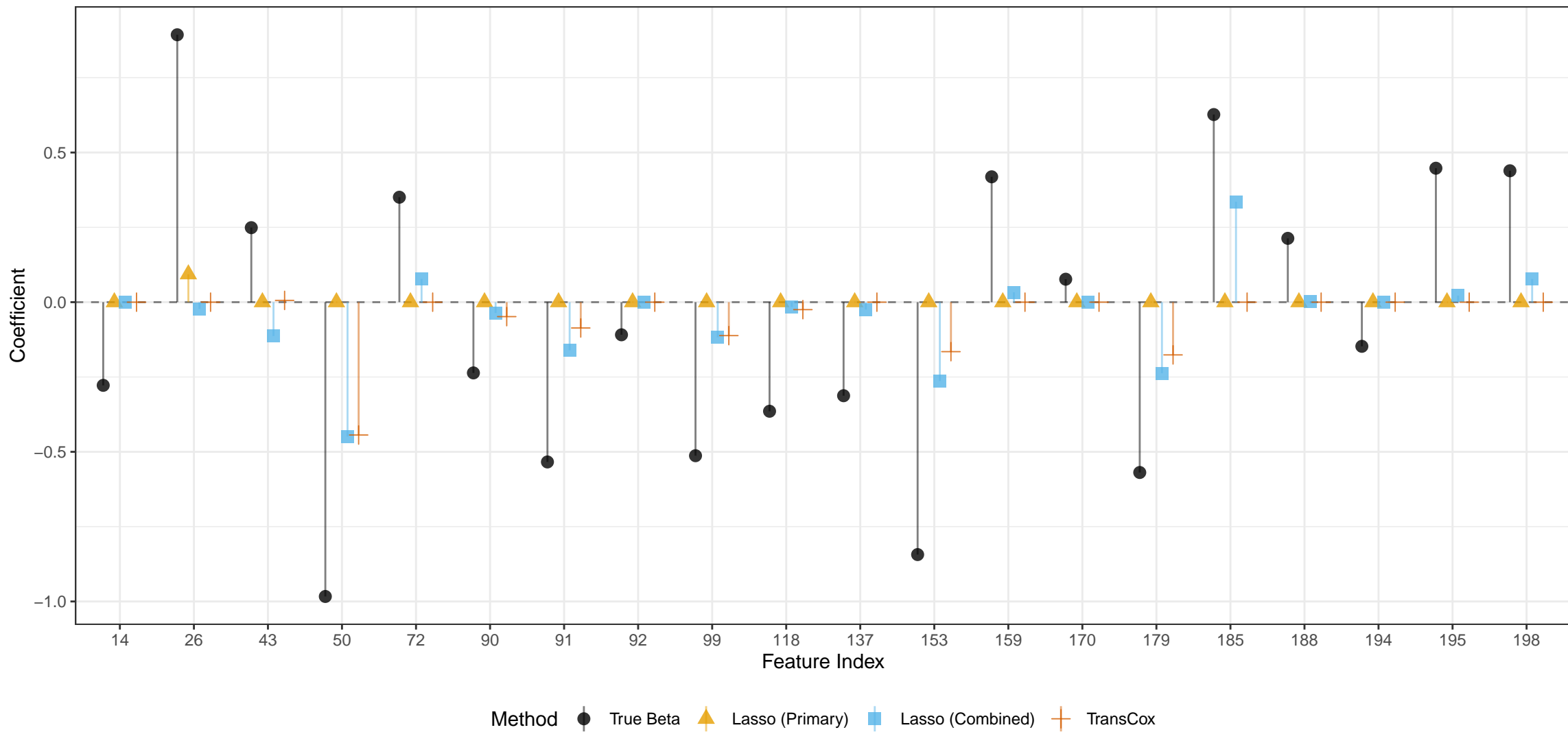
Coefficient Estimation (Active Features)
