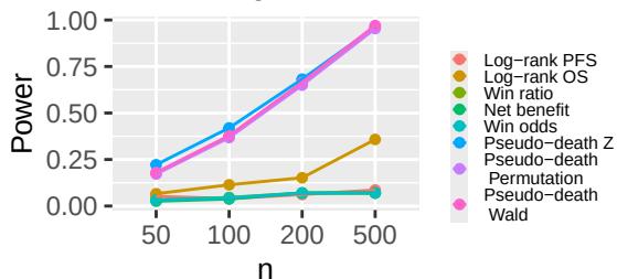
Crossing hazards
