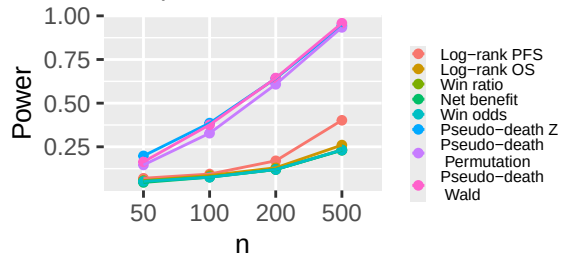
Proportional hazards
