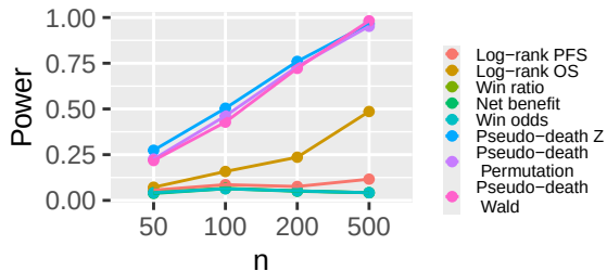
Early difference
