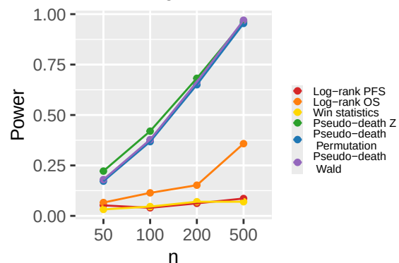
Crossing hazards
