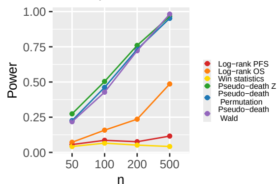
Early difference
