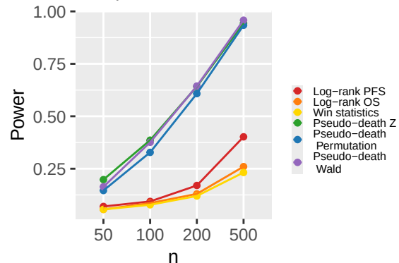
Proportional hazards
