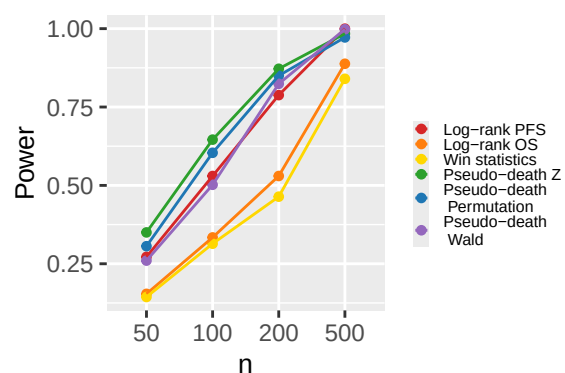
Late difference
