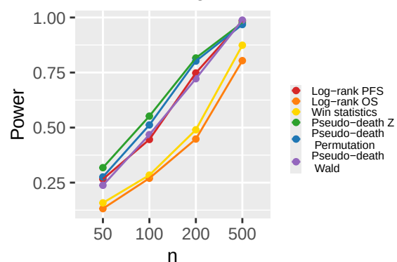
Counteracting effect
