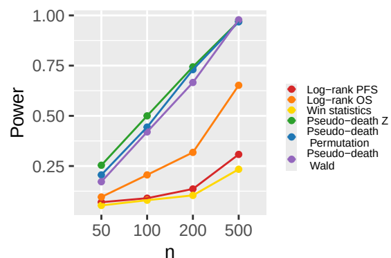
Absent effect
