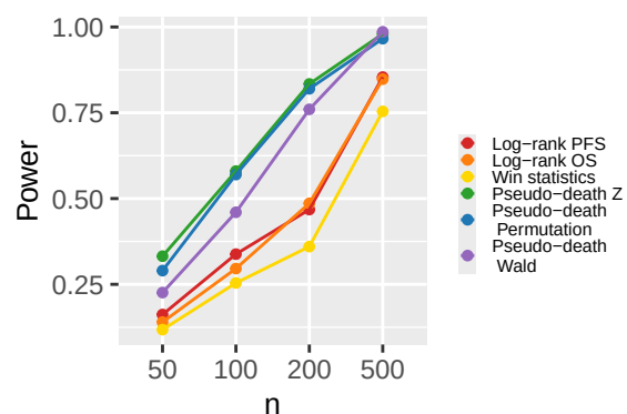
Middle difference
