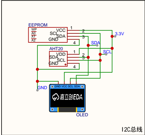
I2C总线
