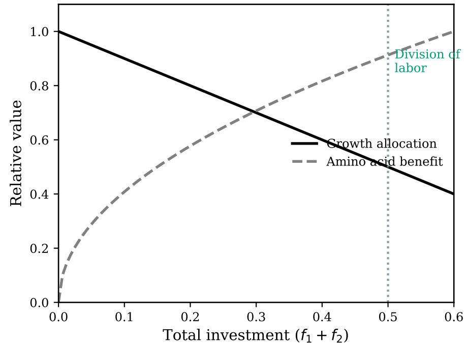
(A) Investment trade-off
