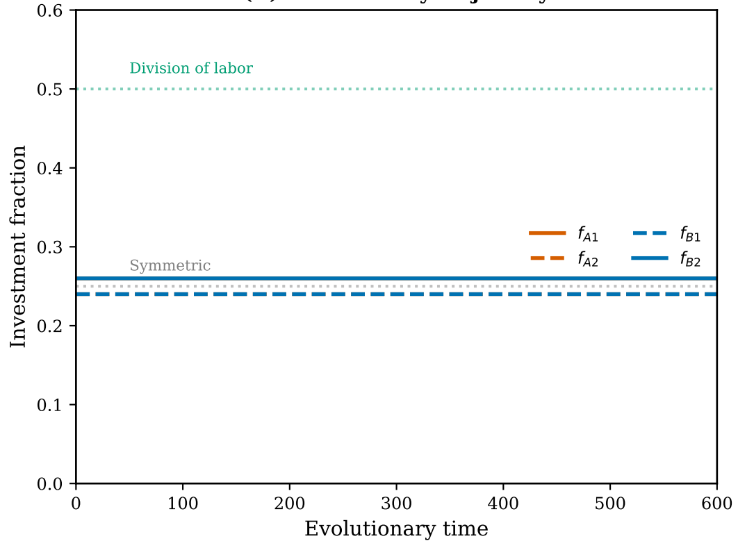
(B) Evolutionary trajectory
