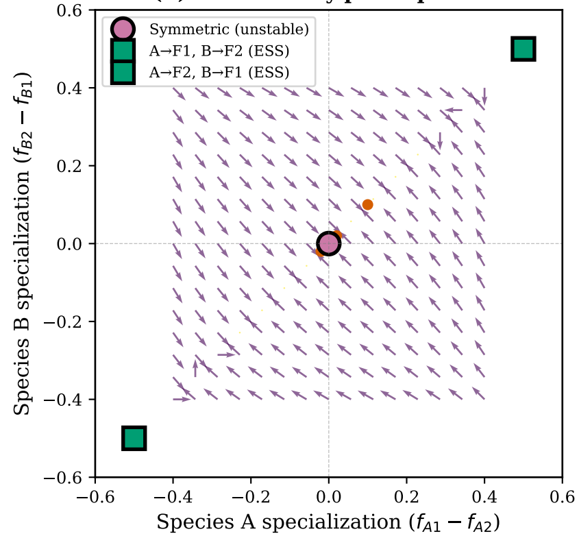
(A) Evolutionary phase portrait
