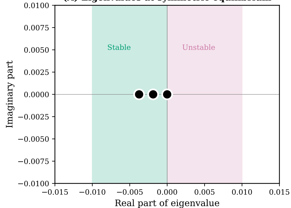
(A) Eigenvalues at symmetric equilibrium
