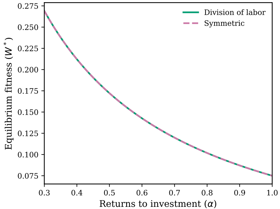
(B) Fitness advantage of division of labor
