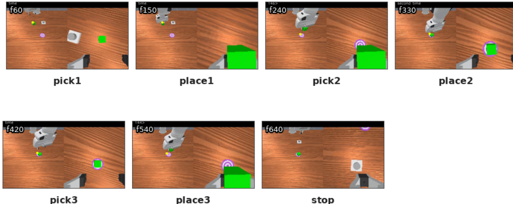
Figure 2: The PickXTimes task: a successful rollout from first pick ( t=60 ) to pressing the stop button ( t=640 ). The robot must pick and place the cube N times and then stop; scenes after each repetition are nearly identical, so progress must be carried by memory.
