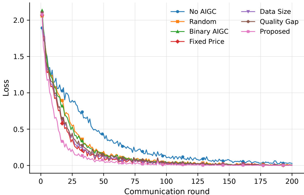
Train Loss vs Communication Rounds
