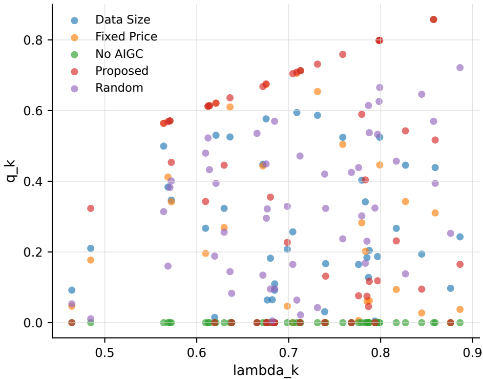
q_k vs lambda_k
