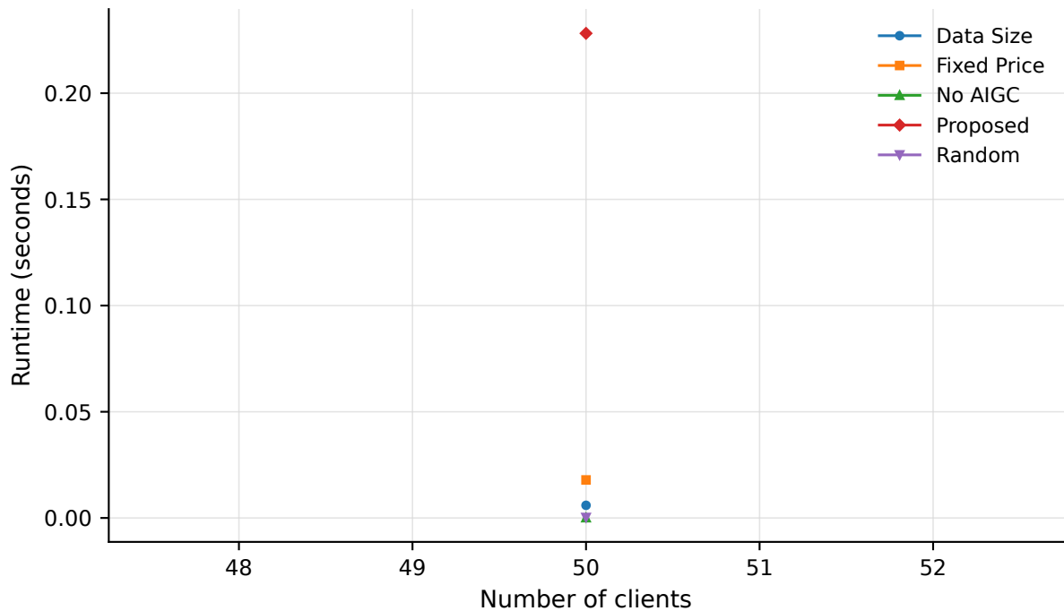
Runtime vs Number of Clients
