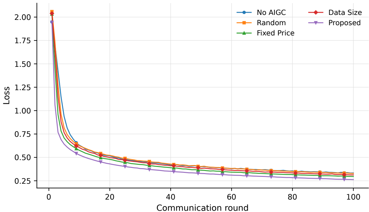
Train Loss vs Communication Rounds
