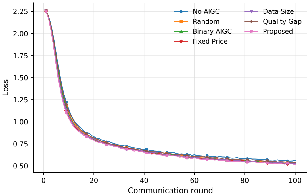
Test Loss vs Communication Rounds
