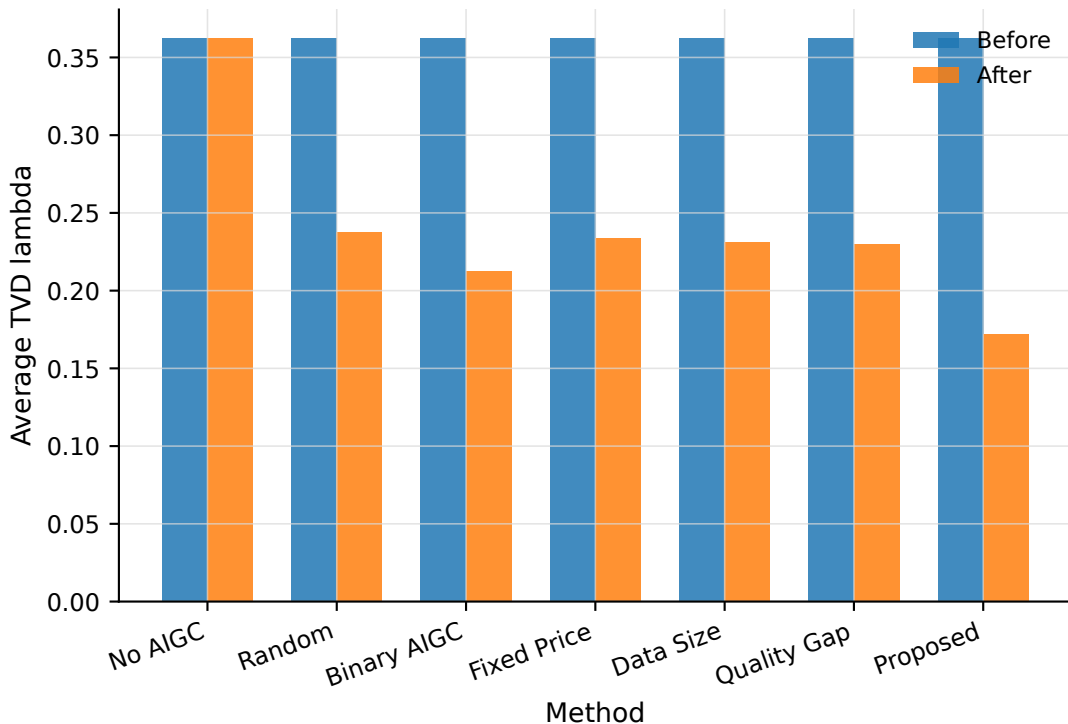
Lambda Before vs After AIGC-Proxy
