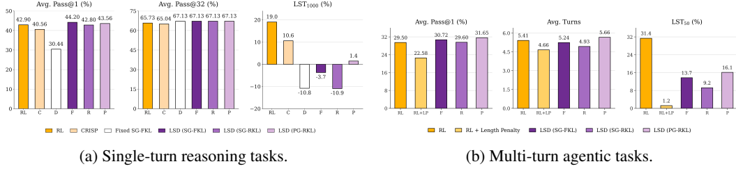
Figure 6: Capability and length-scaling tax across tasks. (a) Single-turn average Pass@1, Pass@32, and LST 1000 . (b) BrowseComp-Plus average Pass@1, turns, and LST 50 . C and D denote CRISP and Fixed SG-FKL; F, R, and P denote LSD with SG-FKL, SG-RKL, and PG-RKL. RL+LP denotes RL + Length Penalty.
