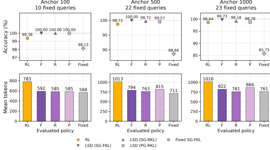
Figure 13: Accuracy and length evaluated on the same fixed queries. Each column uses one RL-frozen cohort with \tau = 1 . The top row reports empirical accuracy; the bottom row reports mean response length. The dashed line marks the 100% anchor accuracy. F, R, and P denote SG-FKL, SG-RKL, and PG-RKL, respectively. Every method is evaluated on the identical query IDs within a column.
