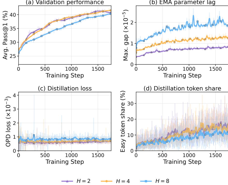
Figure 9: Training signals behind the EMA half-life ablation. All runs use SG-FKL and \tau = 1 . Faint lines show raw values; marked curves show centered 21-point moving means, using available points at the boundaries. Evaluation points are five training steps apart; the other metrics are logged every training step.
