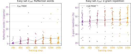
Figure 3: Observable behavior on the fixed easyset. Reflection word frequency and repeated-bigram rate in responses generated by subsequent checkpoints for the same queries in \mathcal{E}_{100} .
