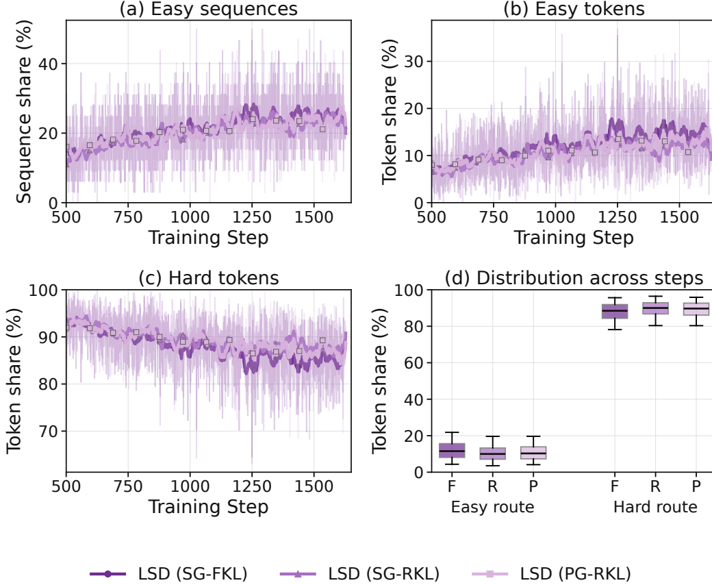
Figure 12: Training token allocation between the easy and hard routes. Panels (a)–(c) show raw per-step fractions and centered 21-step means. Panel (d) summarizes the distribution of token shares across training steps: boxes show the interquartile range and median, and whiskers show the 5th and 95th percentiles. F, R, and P denote SG-FKL, SG-RKL, and PG-RKL. These are distributions of per-step shares, not individual response lengths or uncertainty intervals.
