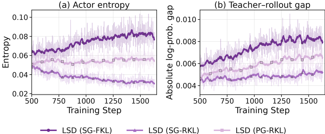
Figure 11: Training dynamics of the three LSD objectives. Actor entropy (left) and the mean absolute teacher–rollout log-probability difference before updates (right) over the shared steps 501–1628. Faint traces show raw per-step values; marked curves show centered 21-step means, using available points at the boundaries. SG-RKL exhibits lower entropy and a smaller teacher–rollout discrepancy over this interval. Each trajectory uses its own run’s training batches.
