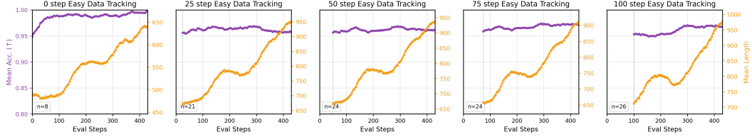
Figure 2: Easy-query accuracy saturates while response length keeps growing during RLVR. At each anchor b \in \{0, 25, 50, 75, 100\} , we select queries with solve rate at least \tau = 0.875 and freeze the resulting easy set.
