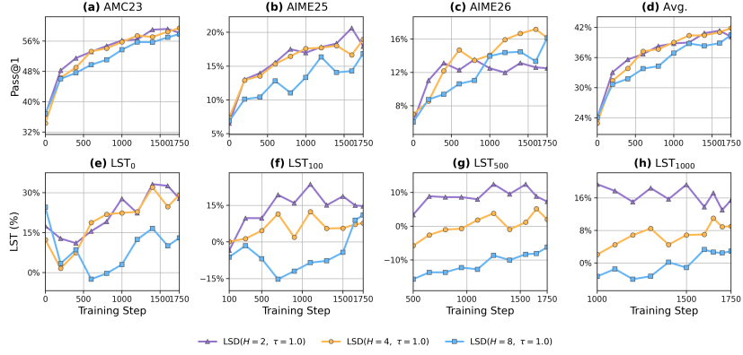
Figure 7: EMA half-life ablation. We compare H = 2, 4, 8 at \tau = 1.0 through step 1750. The upper row shows benchmark and aggregate Pass@1; the lower row shows LST for anchors b = 0, 100, 500, 1000 .
