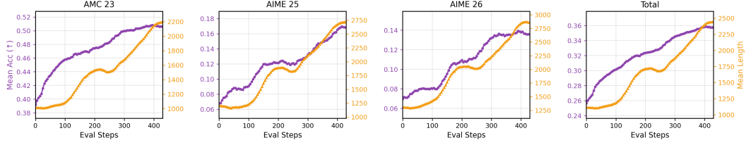
Figure 1: Global validation accuracy and response length during RLVR. Purple circles show mean accuracy, and orange squares show mean response length on three benchmarks and their aggregate over training.
