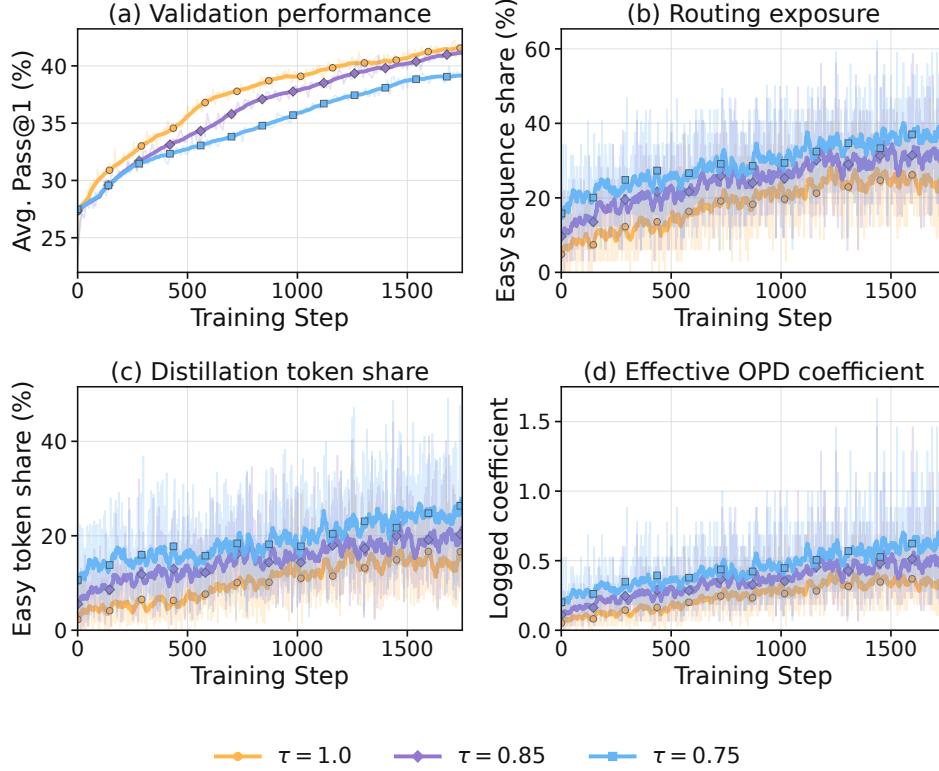
Figure 10: Training signals behind the routing-threshold ablation. All runs use SG-FKL and H = 4 , over steps 1–1750. Raw and smoothed curves follow the convention in Figure 9. Lower thresholds increase the number of sequences and fraction of tokens routed to distillation, as well as the effective OPD coefficient.
