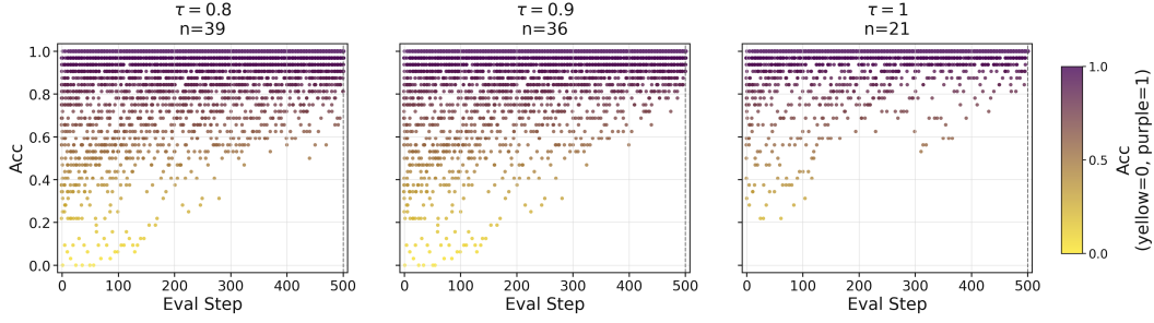
Figure 4: Historical accuracy of prompts selected as easy at step 500. Each point is one prompt at one previous checkpoint. Yellow indicates A(x) = 0 and purple indicates A(x) = 1 .
