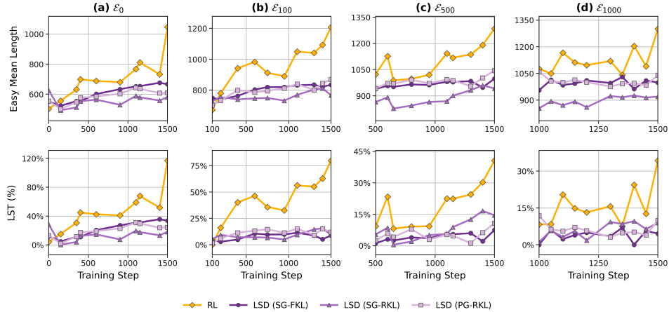
Figure 5: Length growth on fixed easy queries. Across four anchor-defined sets, all three LSD variants have lower easy-query length and LST than RL through most of training. The upper panels report mean length and the lower panels report LST. Different anchors select different cohorts.
