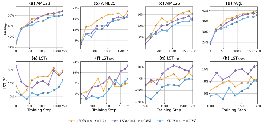
Figure 8: Routing-threshold ablation. We compare \tau = 1.0, 0.85, 0.75 at H = 4 through step 1750. Panels follow Figure 7.
