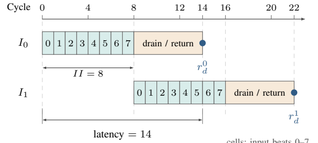
(b) M2: overlapped instruction execution
