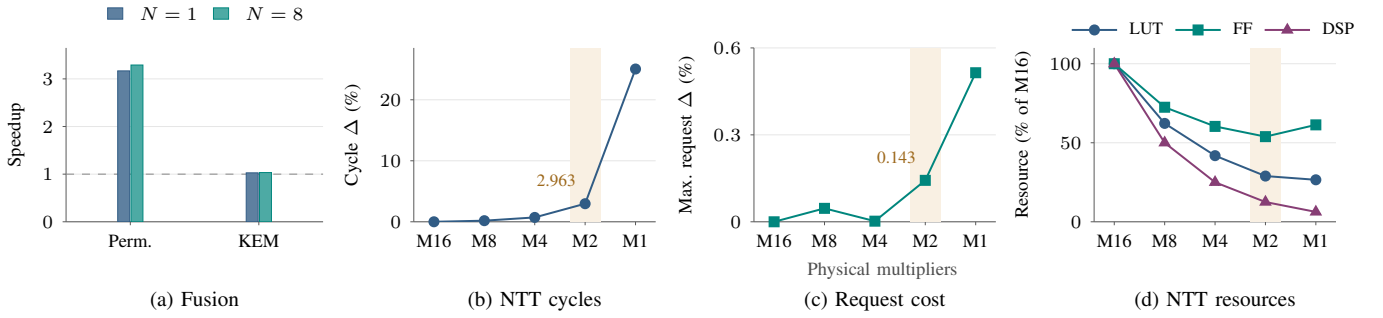
Fig. 5. Controlled granularity and capacity studies. (a) Round/Stage for XRT Keccak intervals and SimX KEM launch cycles, N = 1/8 . (b) Historical W4T32 NTTBF.K test cycles. (c) Maximum W8T32 XRT request overhead across KEM-768/DSA-65 and N = 1/8 , with Pointer Keccak fixed. (d) Independent 200-MHz NTT resources. M16 is the bank reference; gold marks M2.
