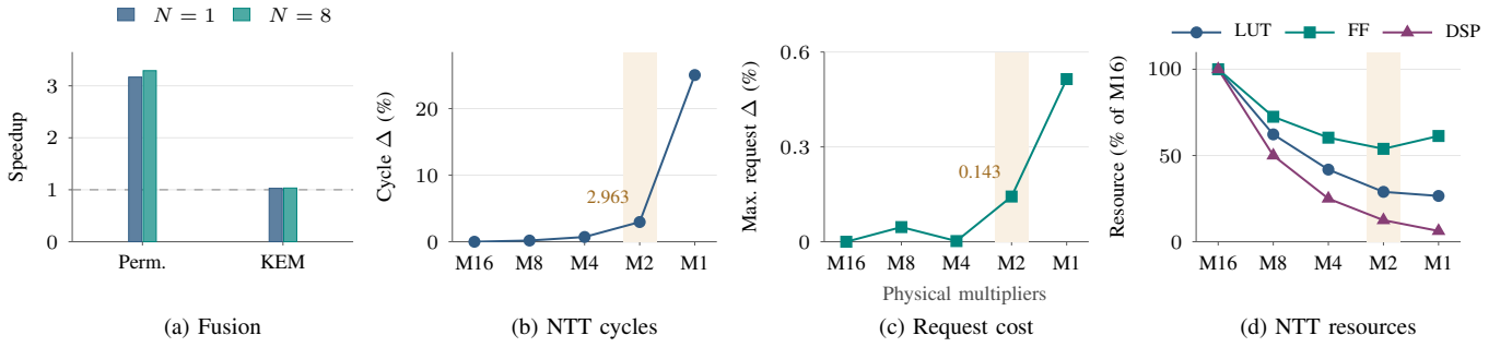
Fig. 5. Controlled granularity and capacity studies. (a) Round/Stage for XRT Keccak intervals and SimX KEM launch cycles, N = 1/8 . (b) Historical W4T32 NTTBFK test cycles. (c) Maximum W8T32 XRT request overhead across KEM-768/DSA-65 and N = 1/8 , with Pointer Keccak fixed. (d) Independent 200-MHz NTT resources. M16 is the bank reference; gold marks M2.
