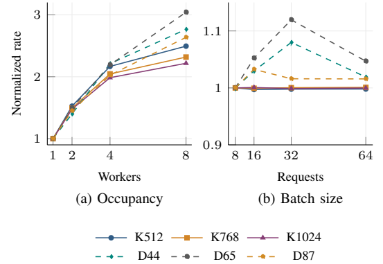
Fig. 6. 200-MHz throughput for E across six sets: (a) eight inputs versus workers, normalized at W = 1 ; (b) batch size at W = 8 , normalized at N = 8 .
