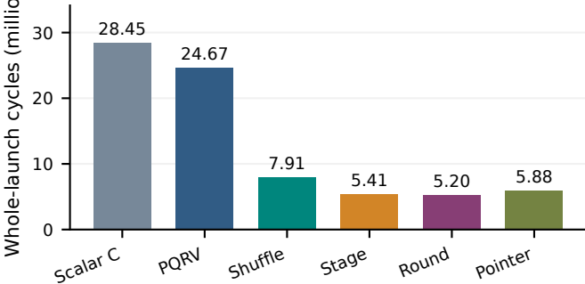
(a) M = 1 request; lower is better
