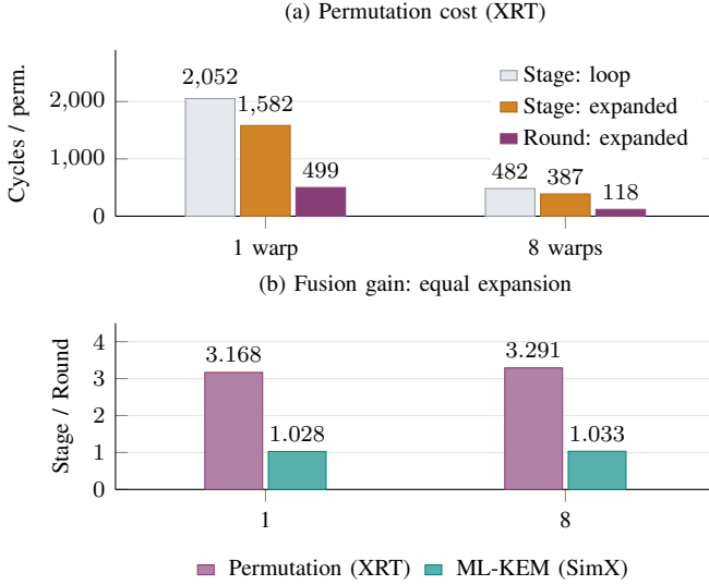
Fig. 7. Keccak granularity with 64 dependent permutations per state. (a) XRT cycles per permutation, one state per active warp. (b) Equal-expansion Stage/Round gain: XRT permutation versus matched SimX complete KEM at one/eight active warps or requests.
