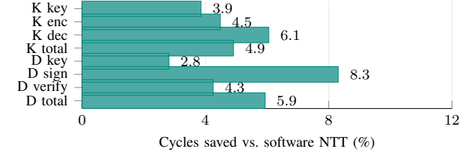
Fig. 8. Complete-request XRT cycle reduction from one shared K/D NTT unit versus W32 register-shuffle software. Pointer Keccak and other arithmetic are fixed within each pair. K: ML-KEM-768; D: ML-DSA-65.
