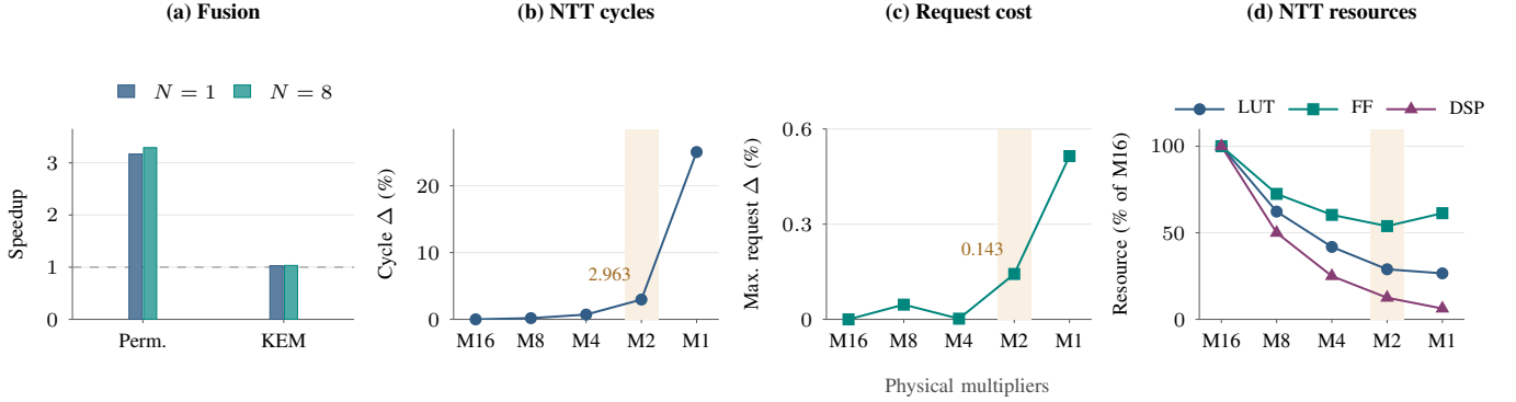
Fig. 4. Controlled granularity and capacity studies. (a) Round/Stage for XRT Keccak intervals and SimX KEM launch cycles, N = 1/8 . (b) Historical W4T32 NTTBF.K test cycles. (c) Maximum W8T32 XRT request overhead across KEM-768/DSA-65 and N = 1/8 , with Pointer Keccak fixed. (d) Independent 200-MHz NTT resources. M16 is the bank reference; gold marks M2.
