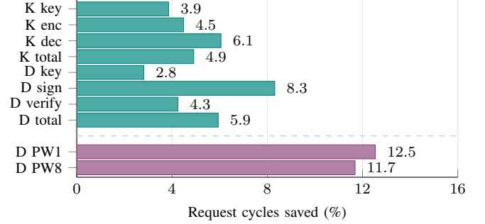
Fig. 8. XRT cycle reductions with Pointer Keccak fixed. NTT bars compare shared instructions with W32 register-shuffle software. PW bars separately compare DSA pointwise mappings with scalar C at M = 1, 8 ; the latter uses batch makespan. K: ML-KEM-768; D: ML-DSA-65. Gains are not additive.
