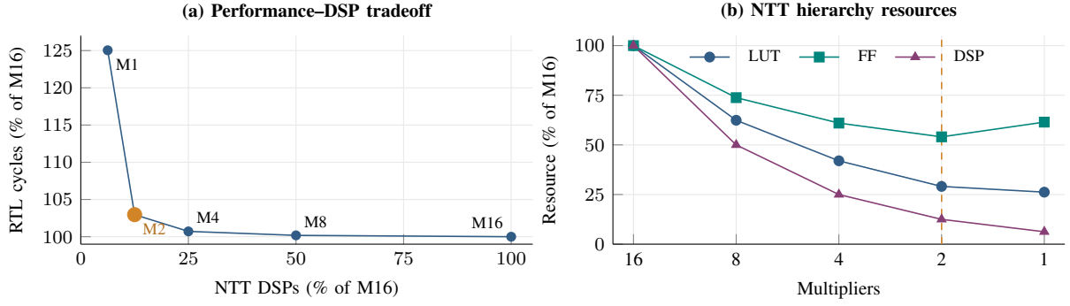
Fig. 9. Matched multiplier-bank sweep. The left panel relates standalone NTTBF.K RTL cycles to NTT-hierarchy DSPs; the right normalizes post-route NTT resources to M16. All five cores close 250 MHz with zero routing errors. Gold marks the selected M2 point.
