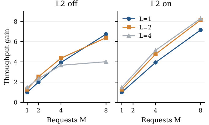
Fig. 2. Historical ML-KEM x4 mapping sweep on 8w \times 4t . Both panels use the sweep’s L2-off, M = 1 , L = 1 baseline of 36,614,668 cycles. Source: mlkem_MxL.csv . These inputs/backend differ from the KAT ablation and the serial-FIPS-202 SG25 experiment.
