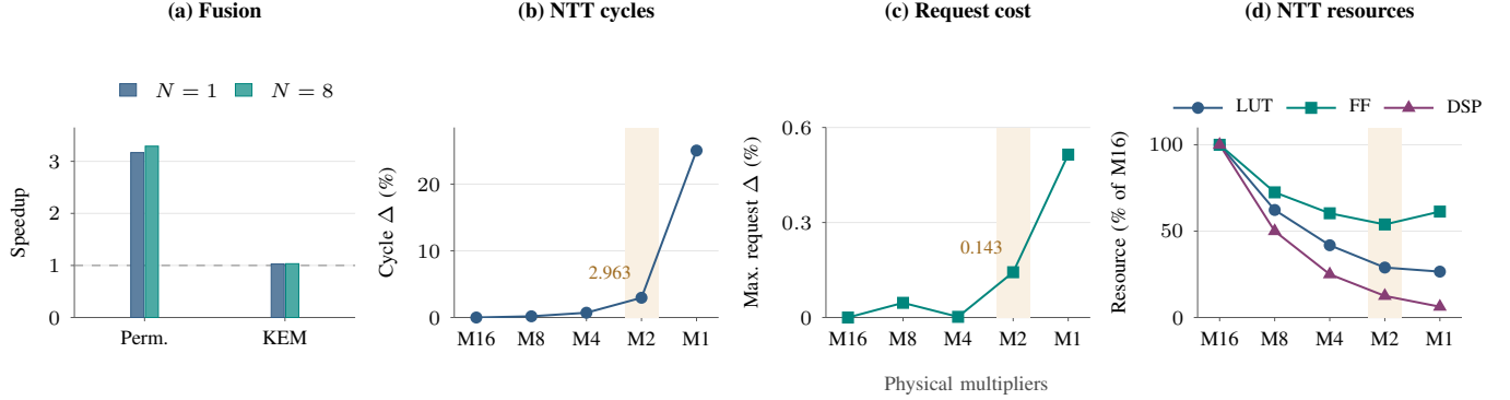
Fig. 4. Controlled granularity and capacity studies. (a) Round/Stage for XRT Keccak intervals and SimX KEM launch cycles, N = 1/8 . (b) Historical W4T32 NTTBFK test cycles. (c) Maximum W8T32 XRT request overhead across KEM-768/DSA-65 and N = 1/8 , with Pointer Keccak fixed. (d) Independent 200-MHz NTT resources. M16 is the bank reference; gold marks M2.
